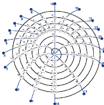
Periodic table: Spiral format by Jan Scholten
